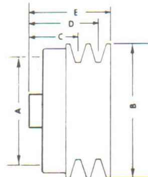
FIG. 3 SELF CONTAINED DOUBLE PULLEY
